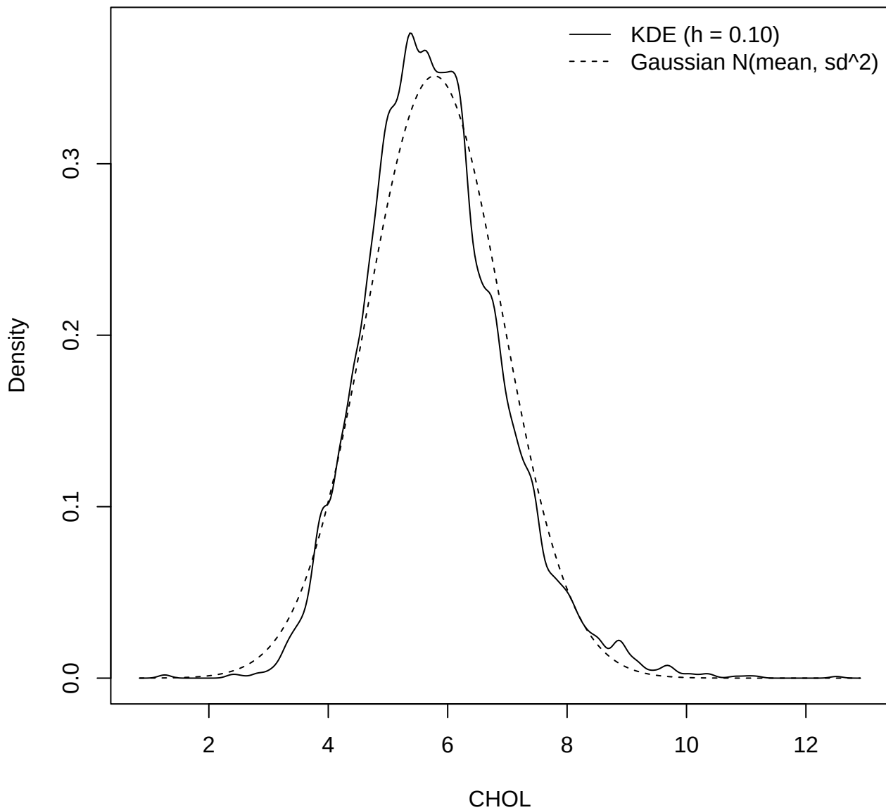
CHOL: KDE (bandwidth = 0.10) vs Gaussian fit
